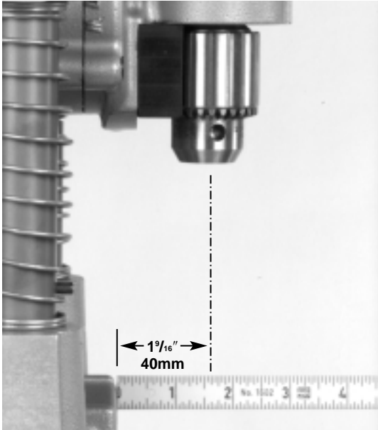
Figure 14 – HC-300 Chuck Centerline
