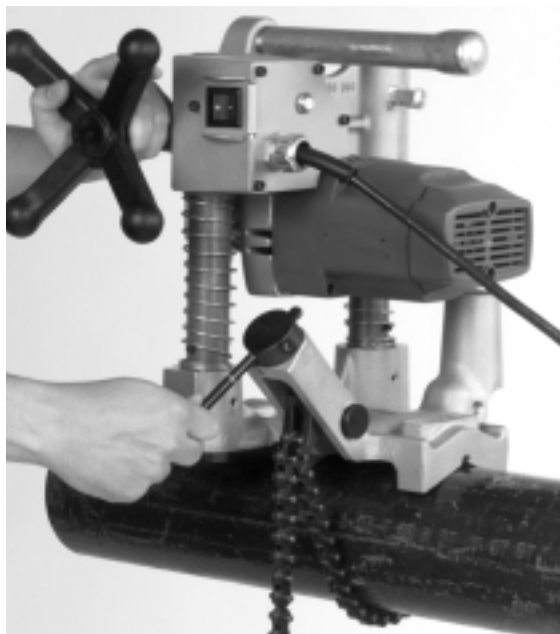
Figure 16 – Tightening Chain
